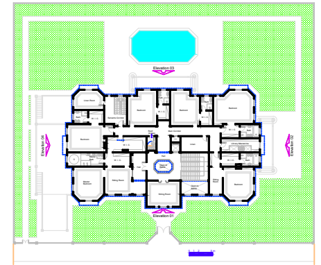
Second Floor Plan A = 508,72 m 2
