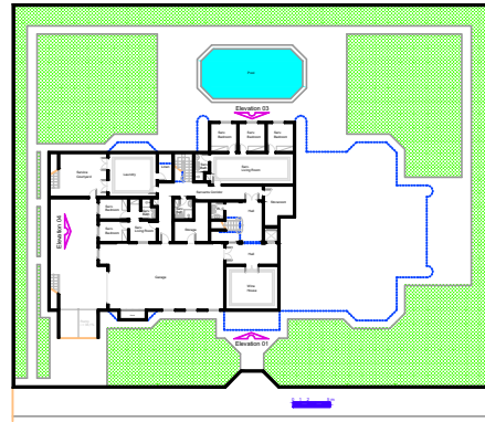
Lower Floor Plan A = 348,31 m 2
